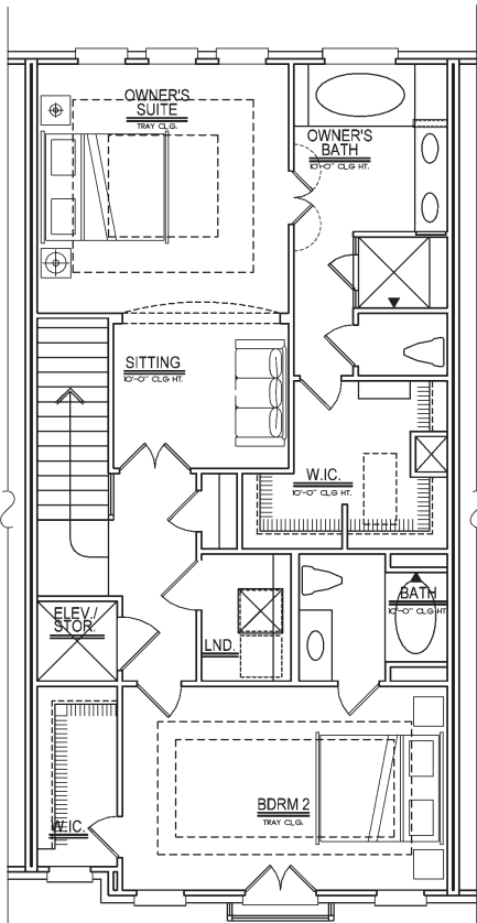
THIRD FLOOR
